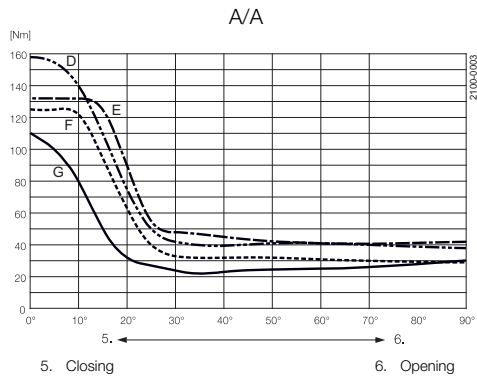
5. Closing 6. Opening
