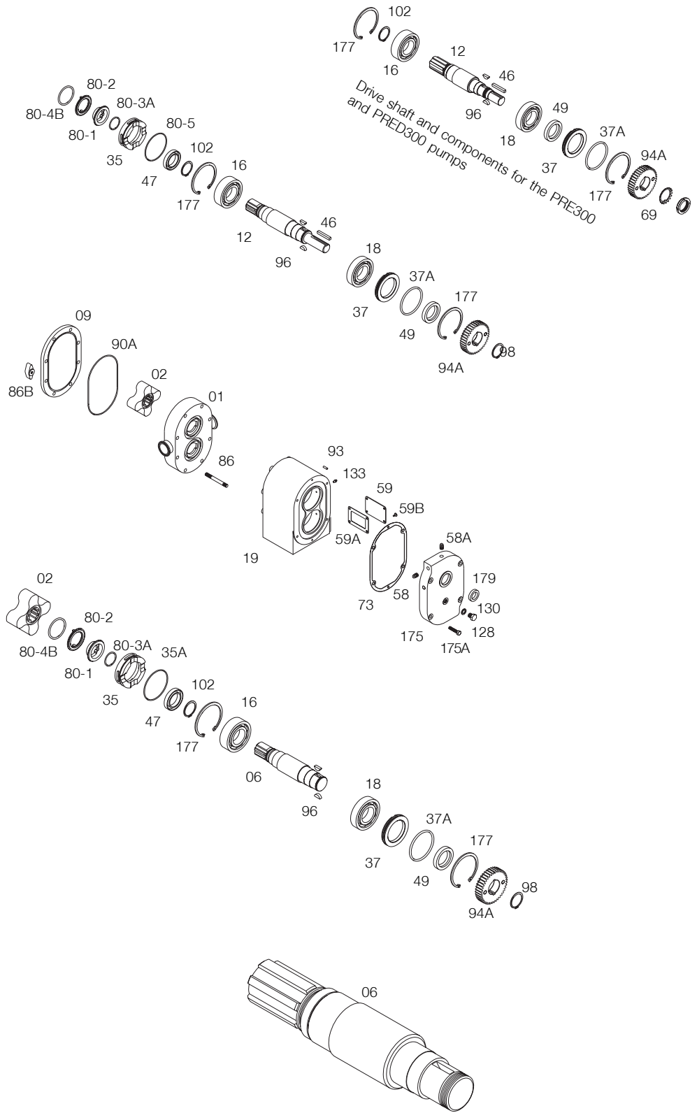
Pump shaft for PRE300 and PRED pumps
