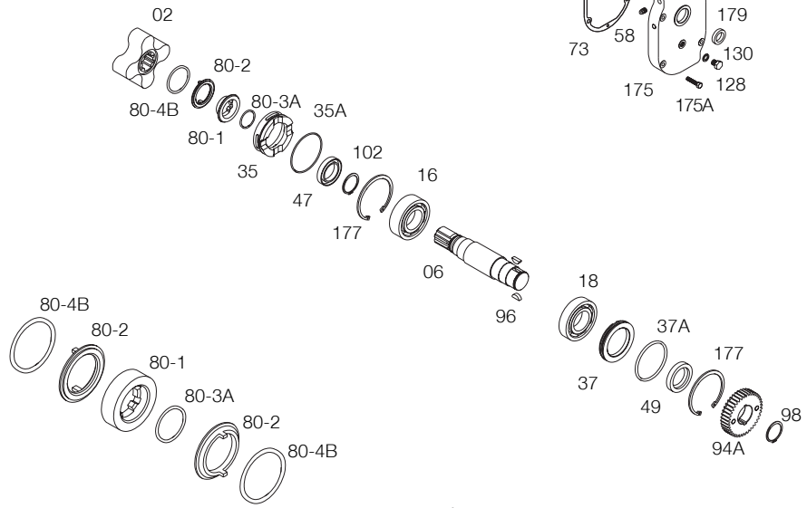
Mechanical seals for PRED pumps
