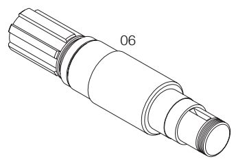
Pump shaft for PRE300 and PRED pumps
