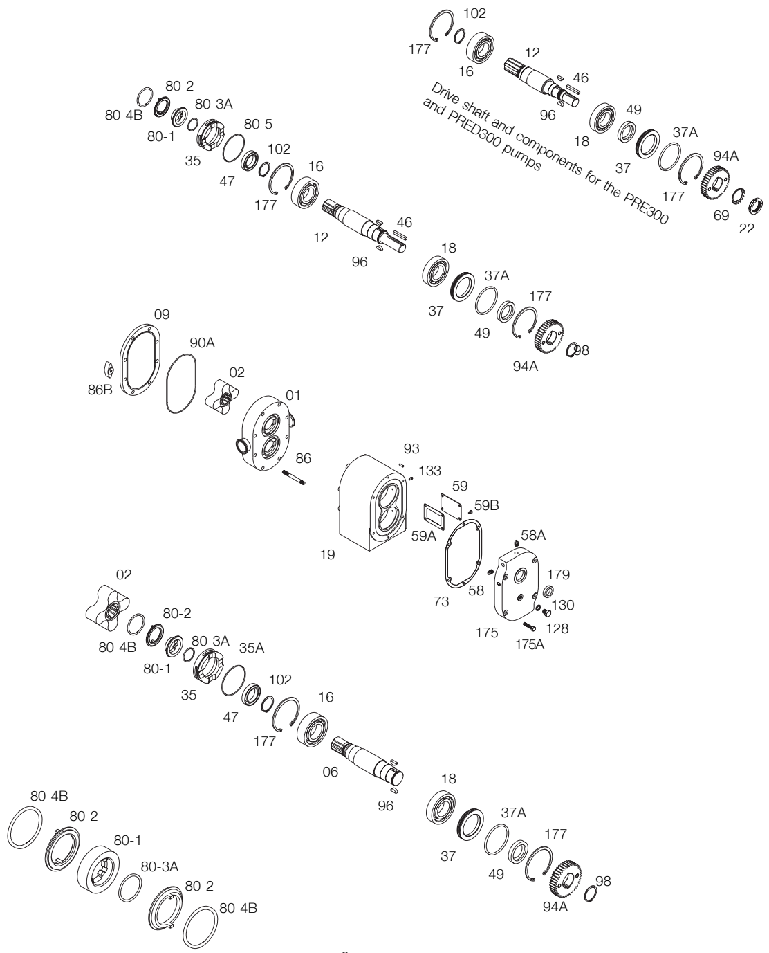
Mechanical seals for PRED pumps
